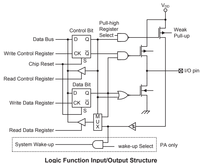
Logic Function Input/Output Structure
